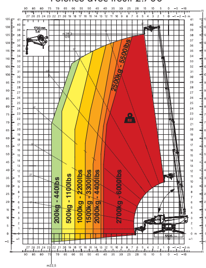
REP 2-4,5 Nacelle extensible rotative 500 kg
