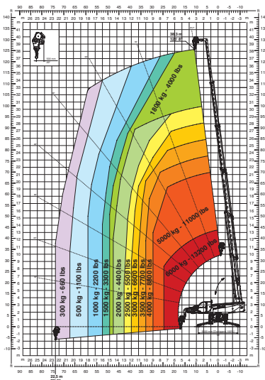
W 6 Treuil 6 tonnes
