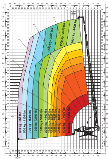
W 6 Treuil 6 tonnes
