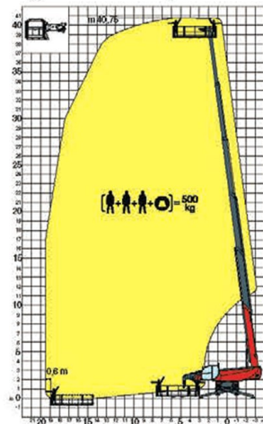
REP 2.2 Rotating fixed platform 500 Kg
