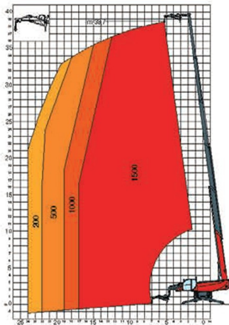
JW 1500 Jib winch 1.500 kg
