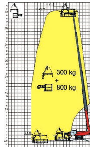
REP 8.2 - 4,7 W0,3 Platform 4,7 m 800 kg with winch 300 kg
