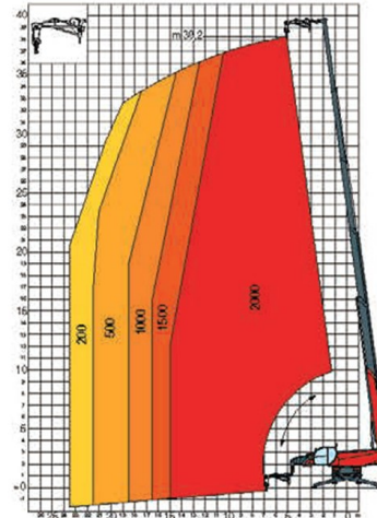
JW 2000 Jib winch 2.000 kg
