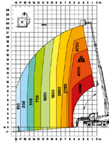
W 5 crochet 5 tonnes
